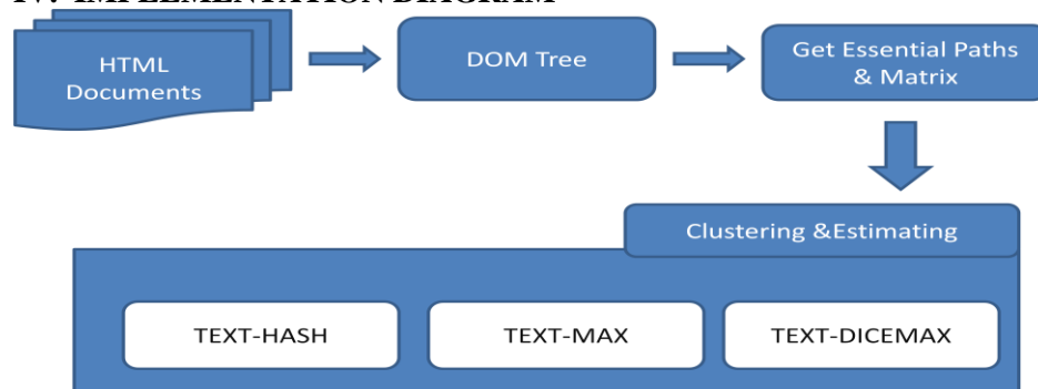
Figure1: System Architecture
