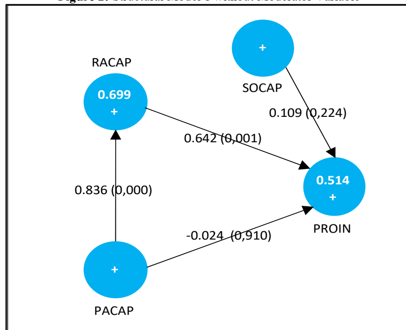
Figure 2: Structural Model 1 without Moderator Variable
