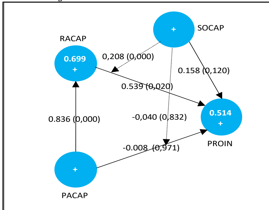
Figure 3: Structural Model 2 with Moderator Variable
