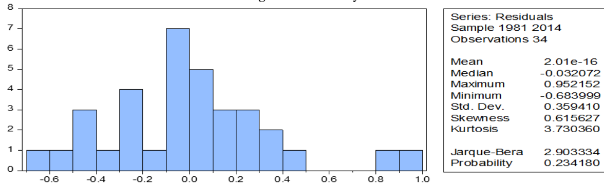
Figure 1: Normality test
