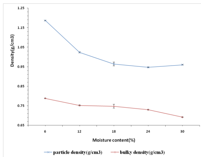
Figure 6 Effect of moisture content on the densities of coffee beans
