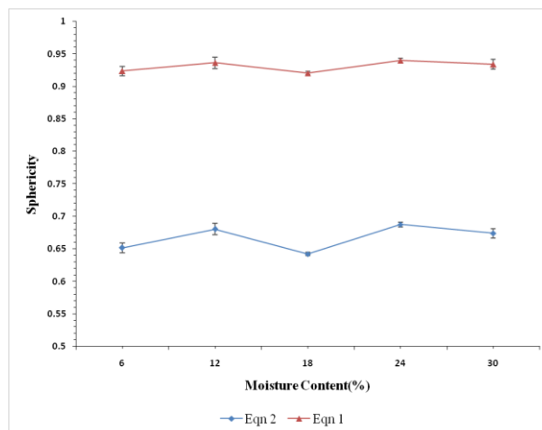
Figure 8 Effect of moisture content on the sphericity of beans
