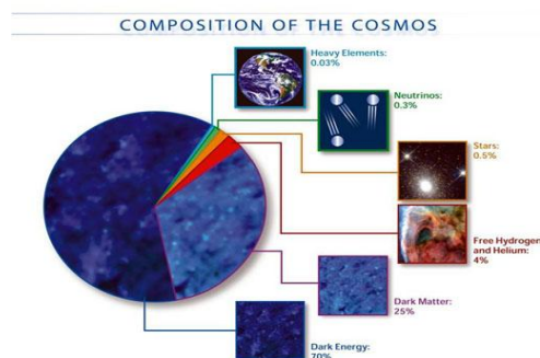
Figure reproduced from the Dark Energy Home Page
