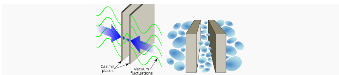
Casimir effect and vacuum energy fluctuations:
