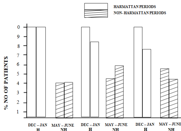
FIG. 5: INCIDENCE OF CORNEA DISEASES DURING (H) HARMATTAN AND (NH) NON - HARMATTAN PERIODS.
