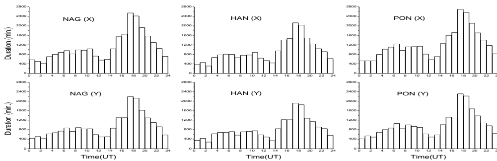
Fig.1 Diurnal variation in Pc4 occurrence at all three stations for the total year 2023.
