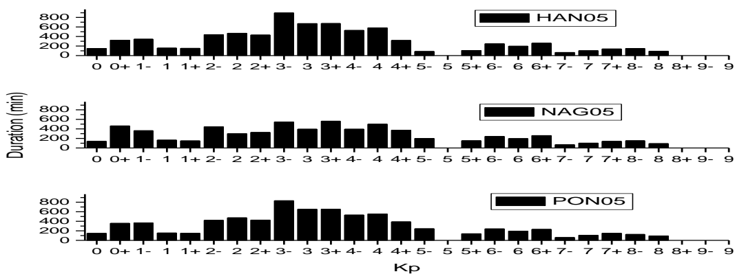
Fig.7: Variation of Pc4 Occurrence (in minutes) with Kp for the winter season of 2023.
