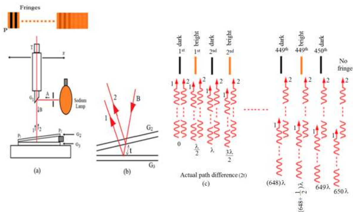
Fig. 3 Ray diagram in Air-wedge method.
