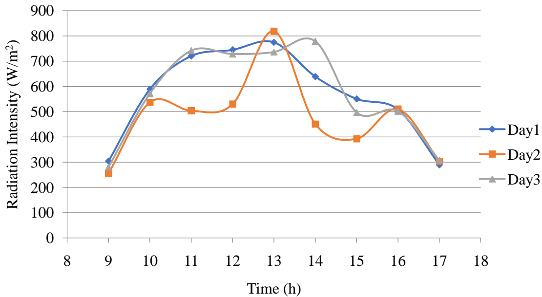
Figure 3 Hourly time variation of solar insolation for day one, two and three.
