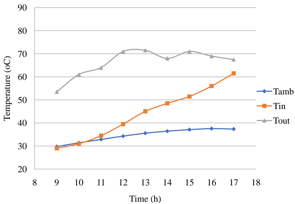
Figure 6. Time variation of Ambient, inlet and outlet temperature for day three.
