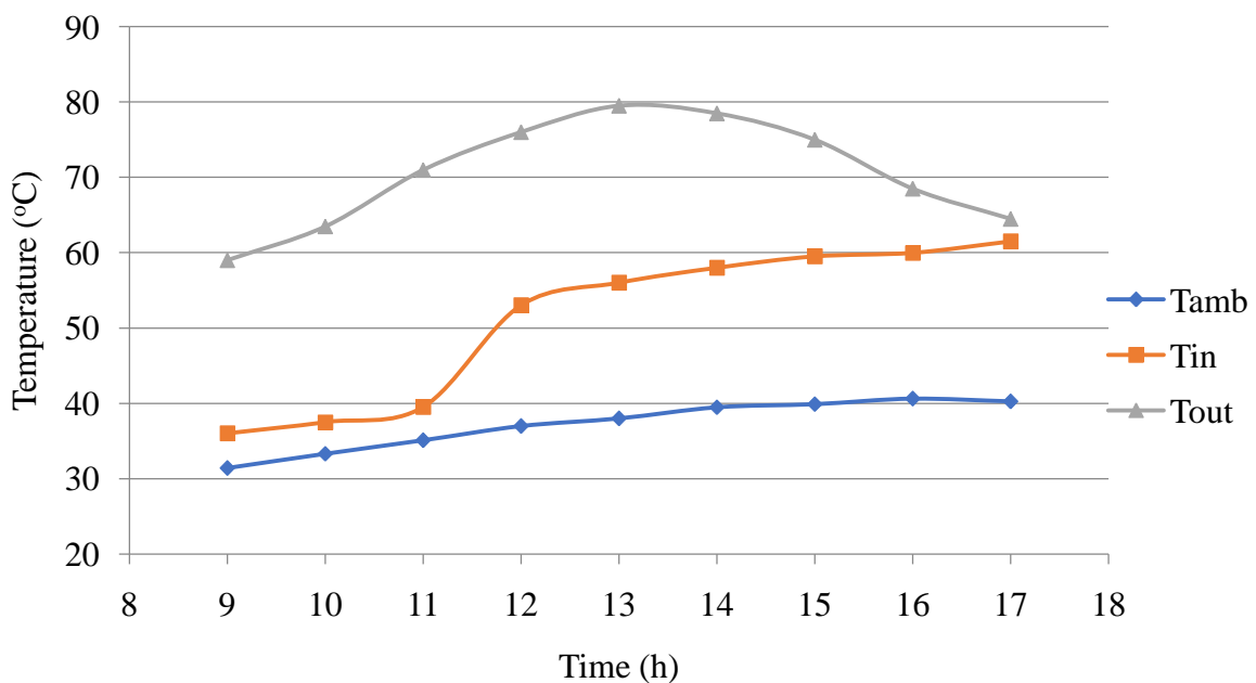
Figure 4. Time variation of Ambient, inlet and outlet temperature for day one.
