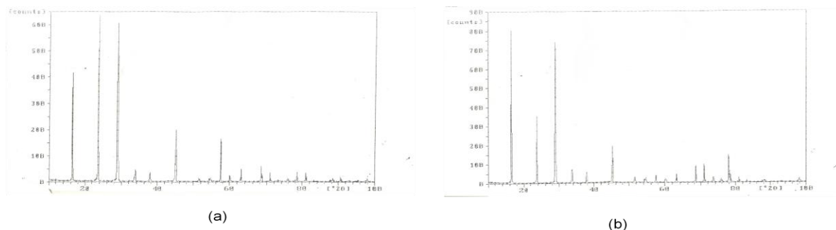
Fig. 3. Powder XRD spectra of (a) pure ADP crystal (b) Glycine doped ADP crystal
