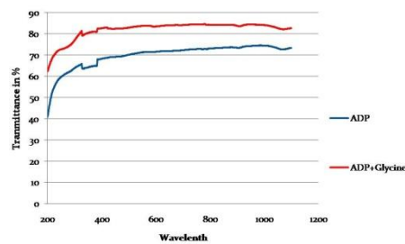
Fig. 4. UV-Vis transmission spectra of pure and doped ADP crystals
