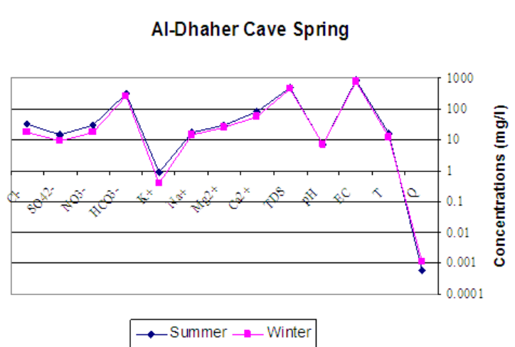
Figure 5. Plot of the samples collected in summer and winter from the Al-Dhaher Cave Spring.
