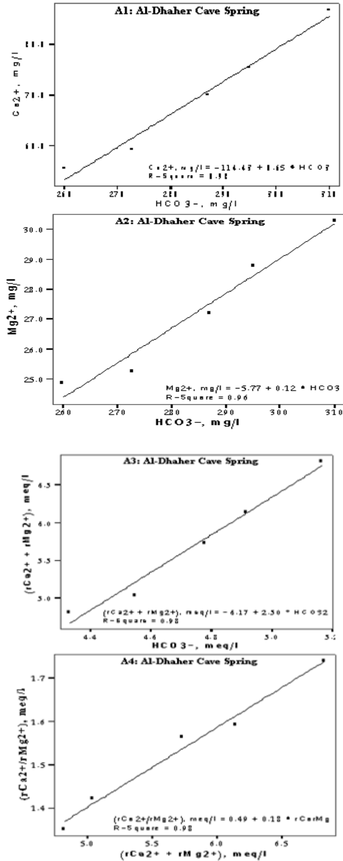
Figure 9. Relation between HCO_3^- and other major cations; (A1, A2, A3, A4) to Al-Dhaher Cave Spring.
