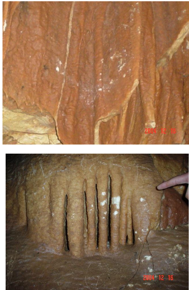
Figure 4. Curtain shape developed from carbonate water trickles down an inclined walls.
