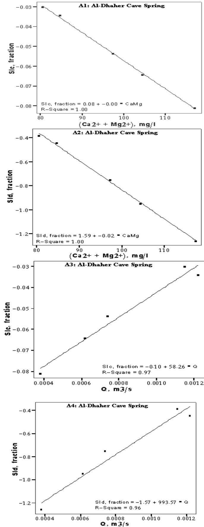
Figure 11. Relation between SI c and SI d versus of (Ca 2+ +Mg 2+ ) and discharge (Q), (A1, A2, A3, A4) to Al-Dhaher Cave Spring.
