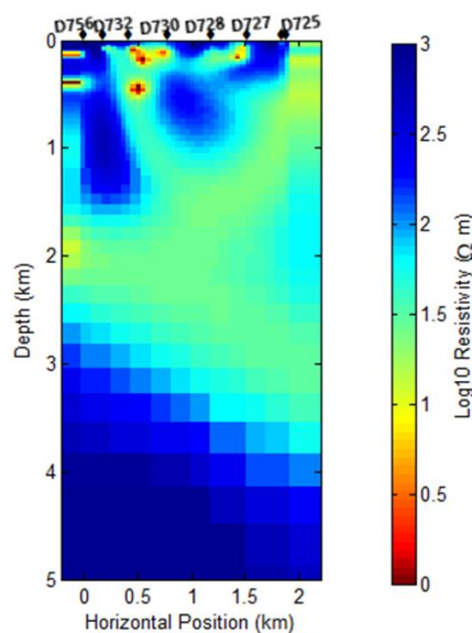
Figure 13: 2D resistivity models for profile 2
