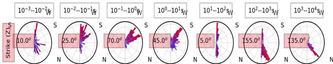
Figure 9: Geo-electric strike rose diagrams of 45° at periods 10 0 – 10 1 s.
