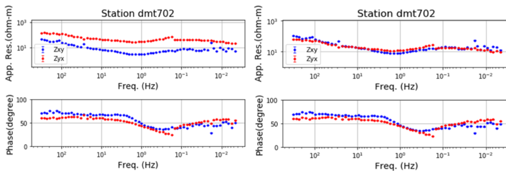
Figure 4: MT data curves before and after static shift and distortion removal.
