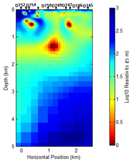
Figure 12: 2D resistivity models for Profile 1
