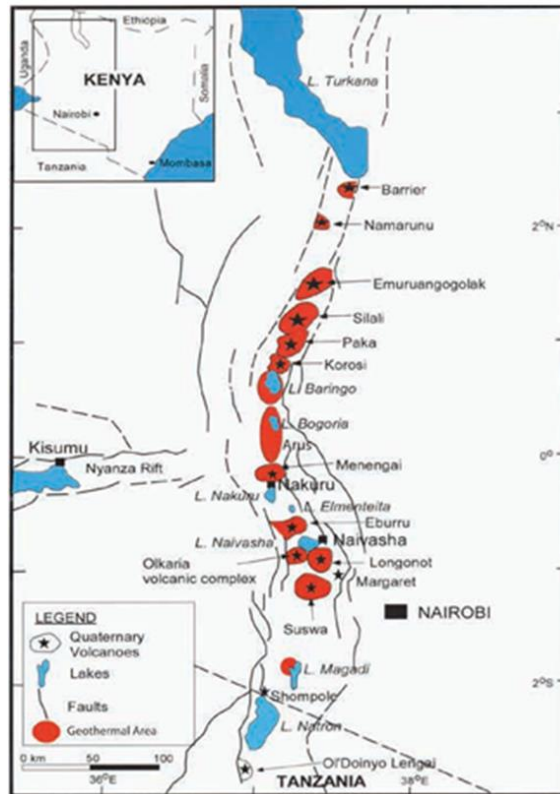
Figure 1: Map of the Kenyan rift system showing the location of potential geothermal prospects (Owona et al. , 2006).
