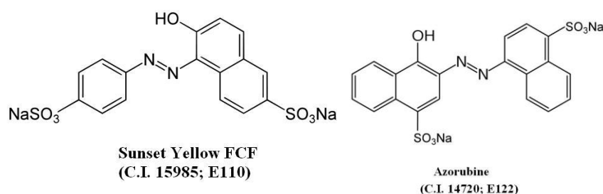
Fig. 1: Chemical structure, name, color index and Enumber of the dyes used.
