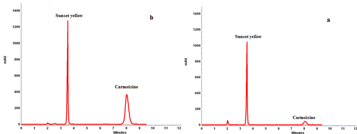
Fig. 2. HPLC-UV-vis chromatogram ( \lambda = 500 nm) sample of soft drink 15 (a) nonspiked and (b) spike of 10 mg L -1 of mixture standard solution of the two dyes
