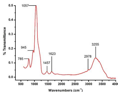
Figure-3 FTIR Spectra of 0.5 M SiNPs
