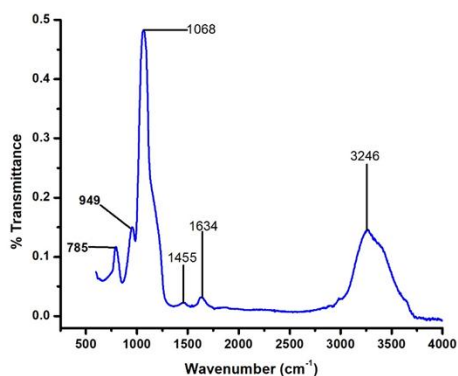
Figure-3 FTIR Spectra of 0.5 M SiNPs
