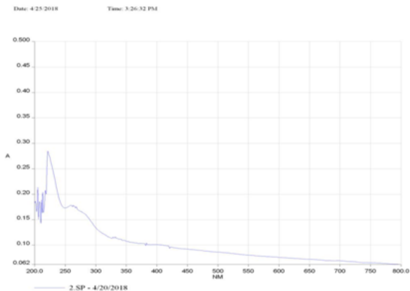
Figure 2: UV Spectra of NiS-SiO 2
