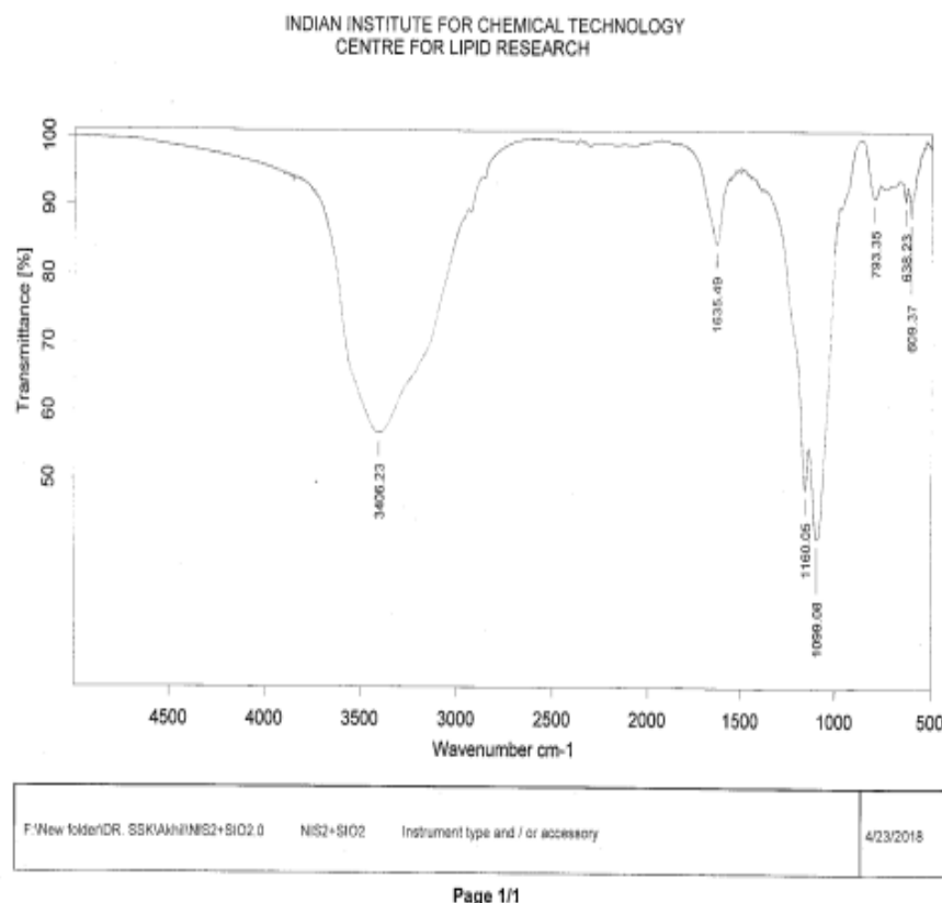
Figure 3: IR Spectra of NiS-SiO 2
