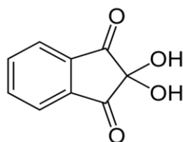
Scheme 2. The chemical structure of ninhydrin.
