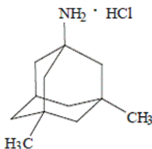
Scheme 1. Structure of memantine hydrochloride (MEM).
